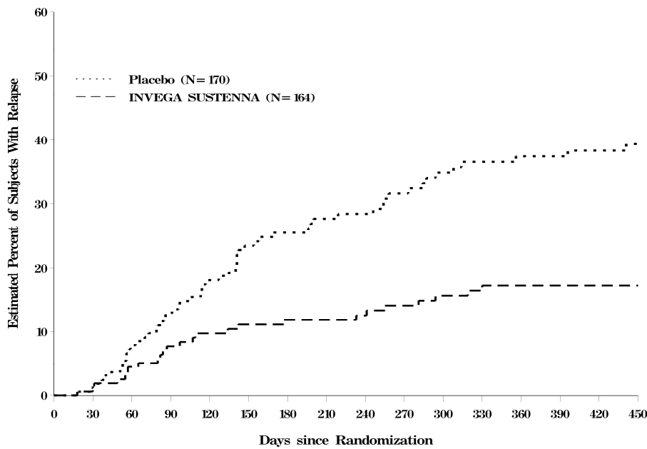
Figure 4: Kaplan-Meier Plot of Cumulative Proportion of Subjects with Relapse Over Time (SAff Study 1)
